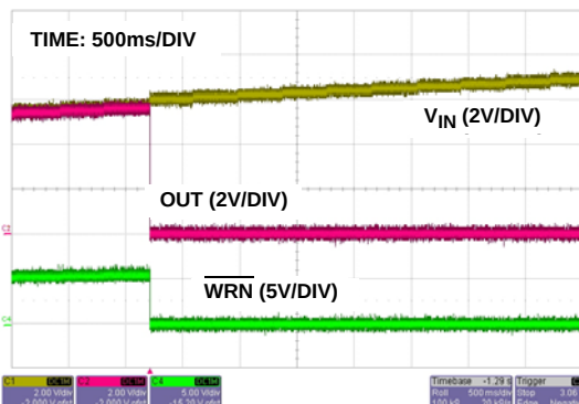
FIGURE 4. CAPTURED WAVEFORMS WHEN THE INPUT VOLTAGE GRADUALLY RISES TO THE INPUT OVERVOLTAGE THRESHOLD
