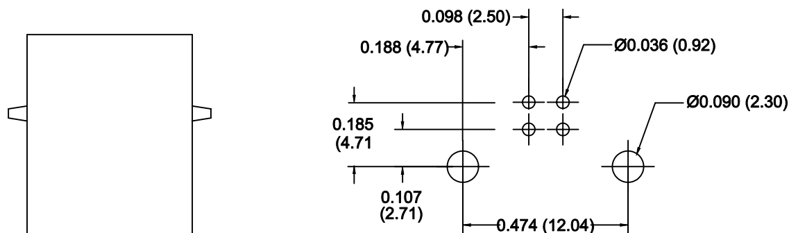
PC BOARD MOUNTING DIMENSIONS
