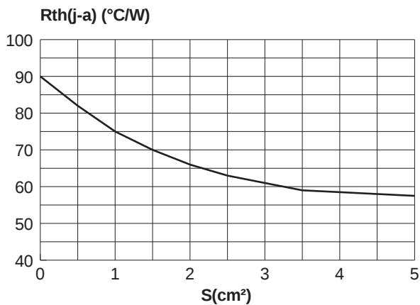
Fig. 8: Thermal resistance junction to ambient versus copper surface under each lead (Printed circuit board FR4, e(\text{Cu})=35\mu\text{m} )
