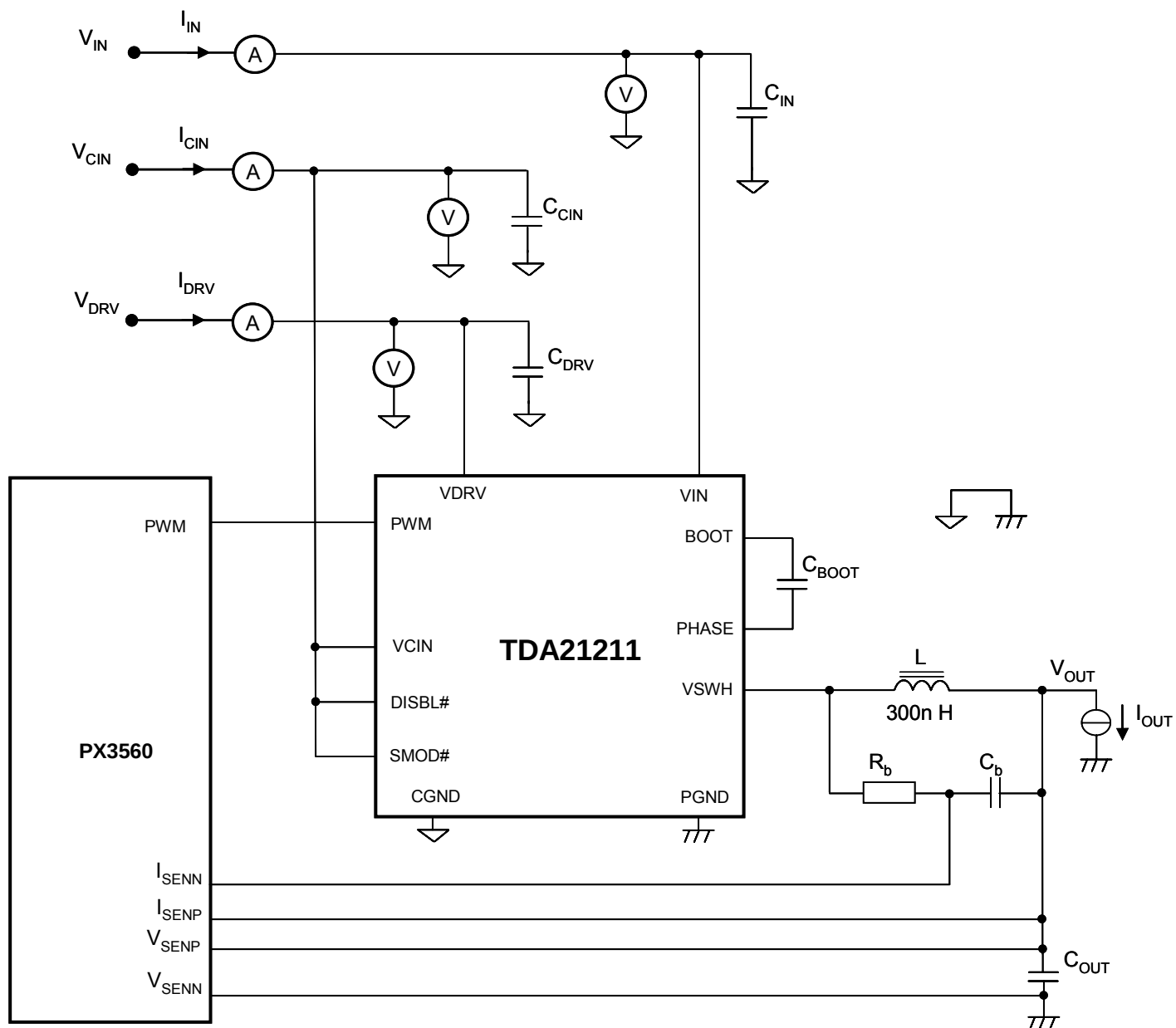
Figure 8. Test Circuit
