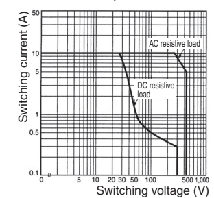
G2RL-1A-H, G2RL-1-H
