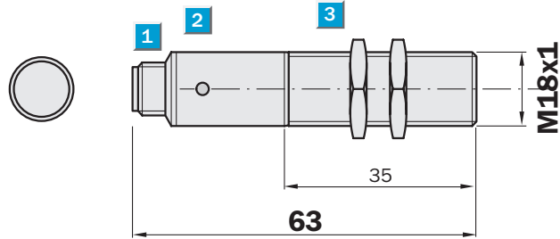
Dimensional drawing
