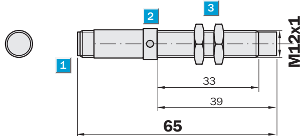
Dimensional drawing
