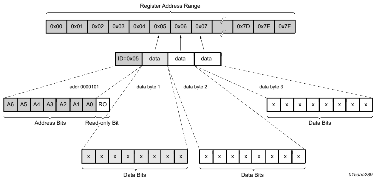
Fig 15. SPI data structure for a write operation (16-, 24- or 32-bit)
