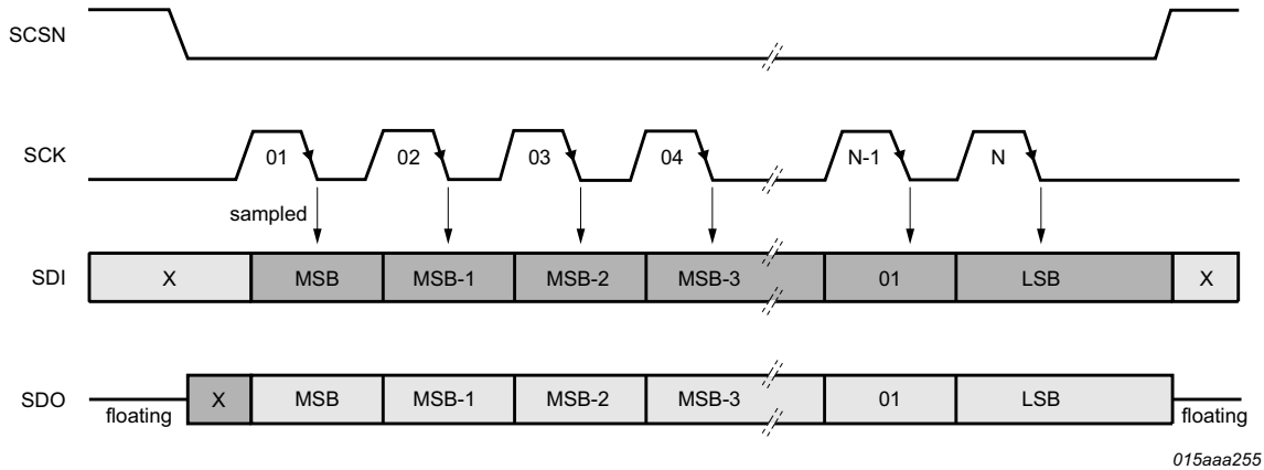
Fig 14. SPI timing overview (see Figure 18 for detailed SPI timing)
