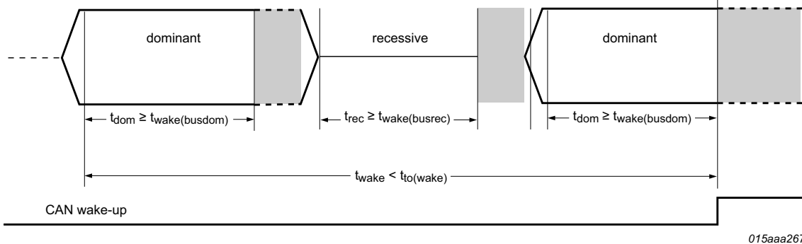
Fig 9. CAN wake-up timing
