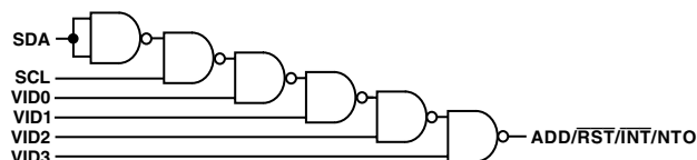
Figure 7. NAND Tree
