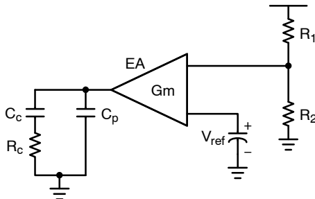
Figure 10. Type II Transconductance Error Amplifier
