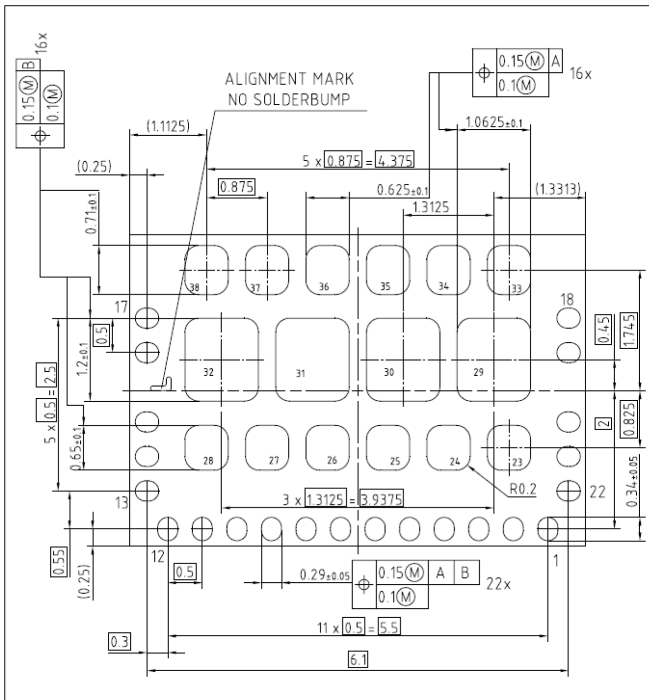
Figure 19 Mechanical Dimensions of Package (Bottom View) in mm
