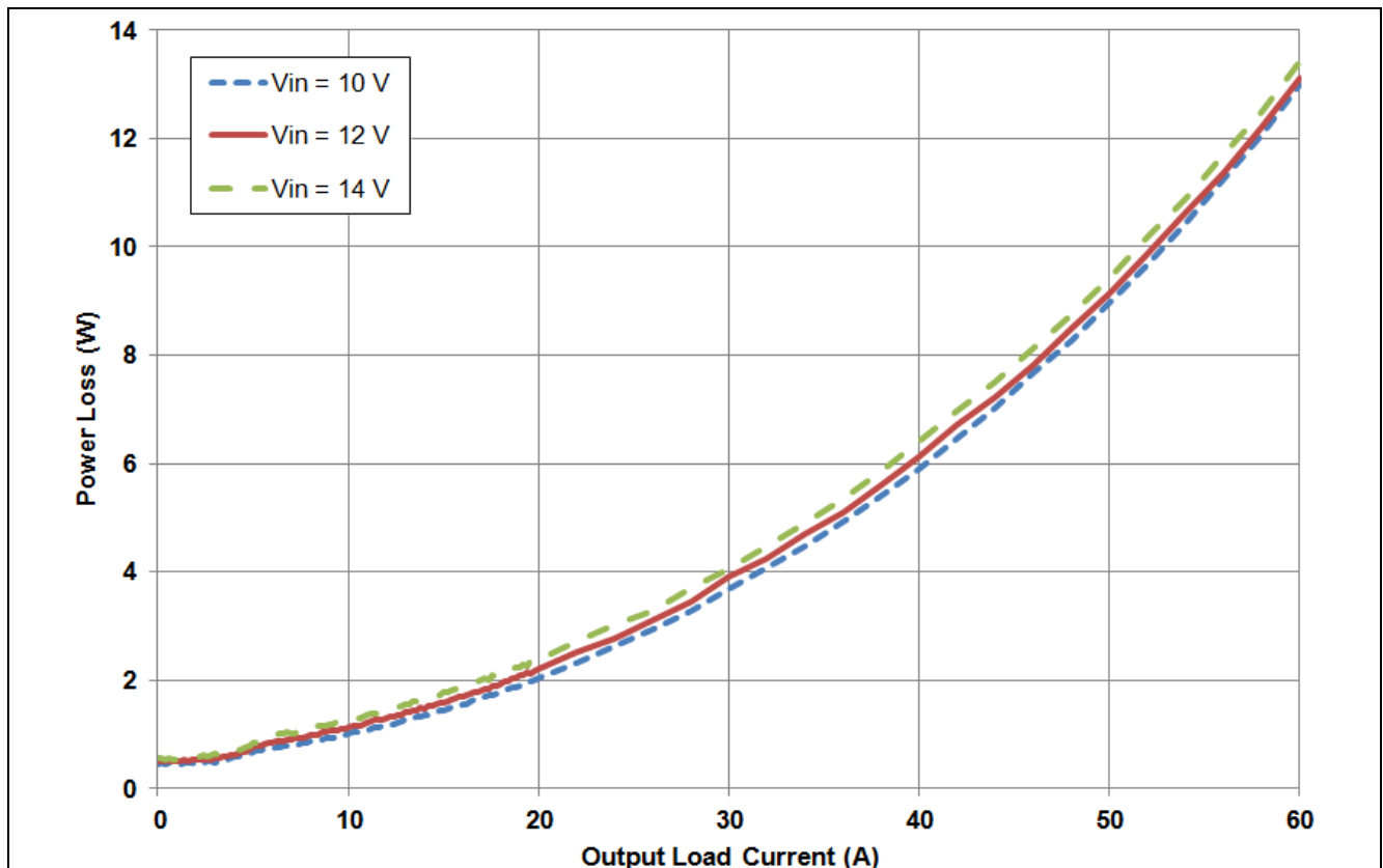
Figure 15 Power Loss at f_{sw} = 750 kHz, V_{cin} = V_{DRV} = 5 V, V_{out} = 1.8 V, Parameter: VIN
