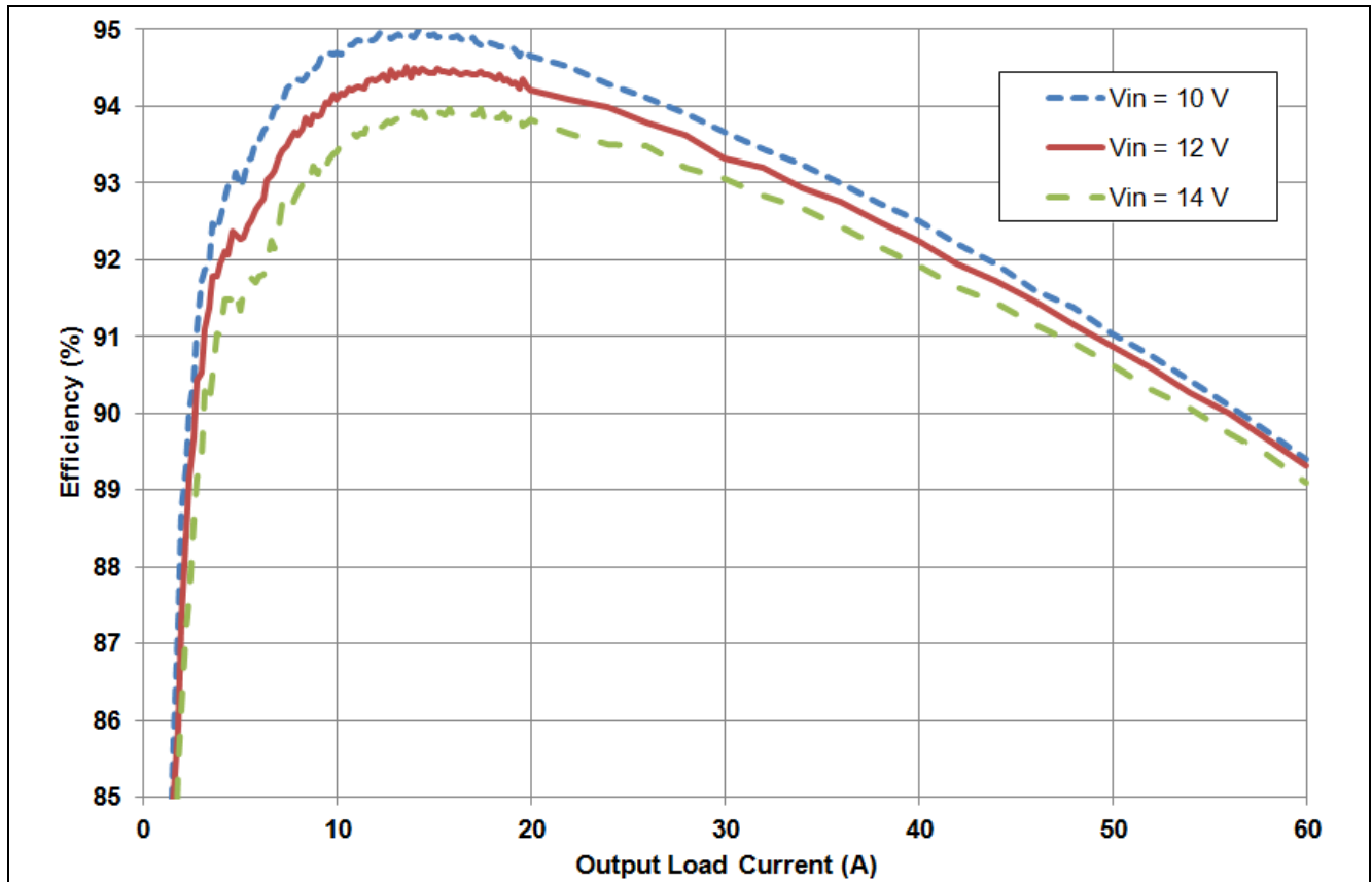
Figure 14 Efficiency at f_{sw} = 750 kHz, V_{cin} = V_{DRV} = 5 V, V_{out} = 1.8 V, Parameter: VIN
