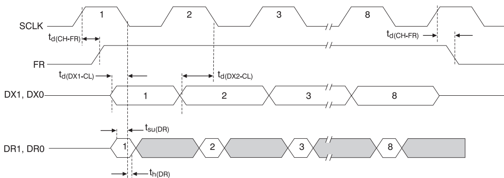
Internal Framing
