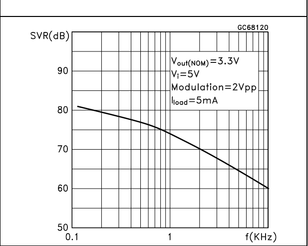
Figure 9. SVR vs. frequency
