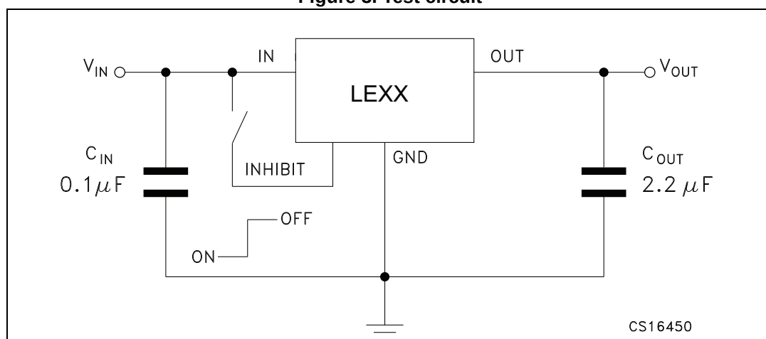
Figure 3. Test circuit
