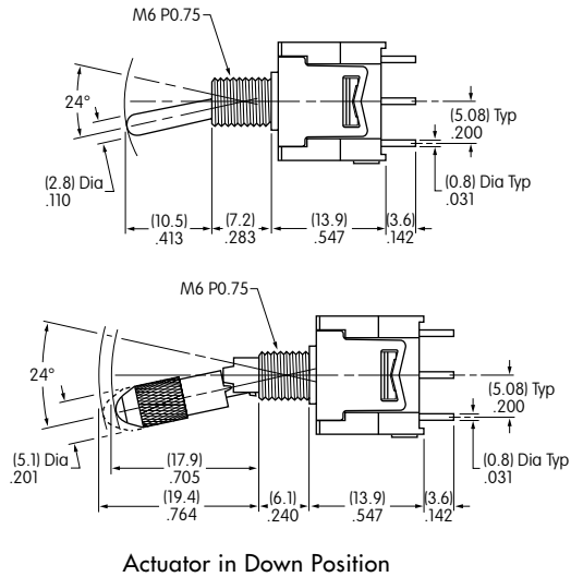
Actuator in Down Position
