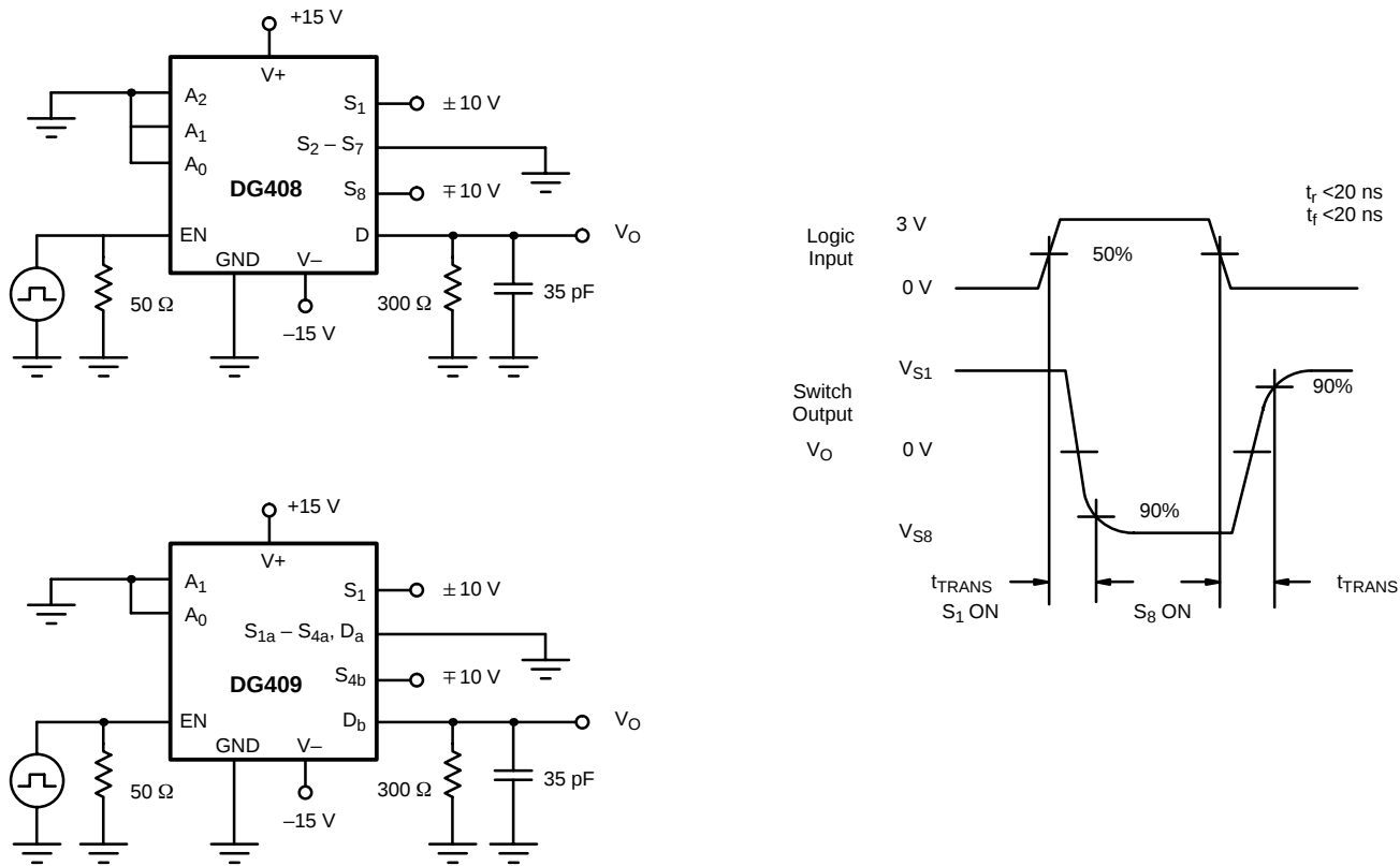
FIGURE 2. Transition Time
