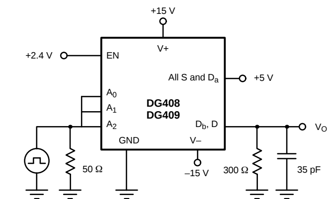
FIGURE 4. Break-Before-Make Interval
