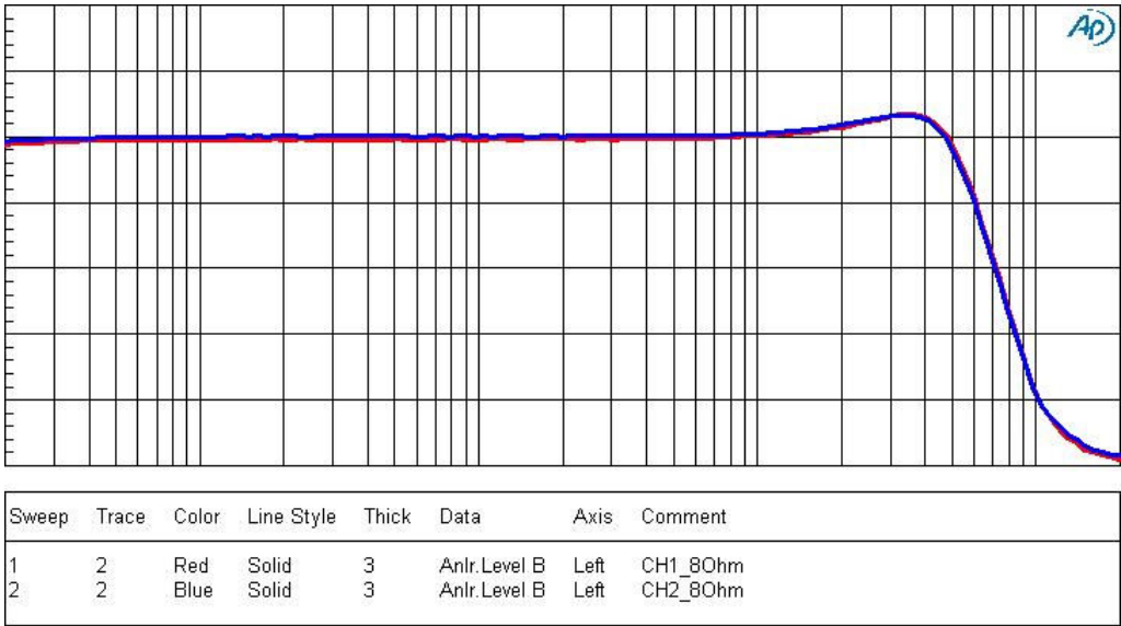
8 ohm load
