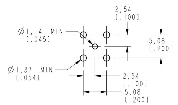
RECOMMENDED PCB MOUNTING HOLE DIMENSIONS SCALE 2.000
