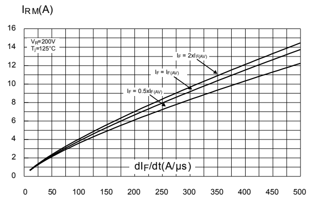
Figure 2. Peak reverse recovery current versus dl_F/dt (90% confidence)
