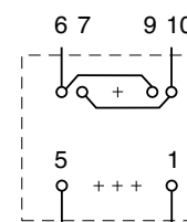
Recommended layout for transformers with 1 secondary winding
