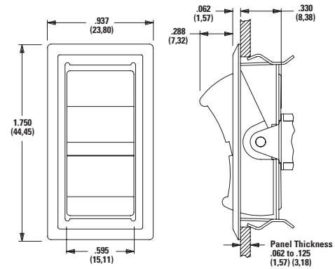
J37 Rocker with Frame
