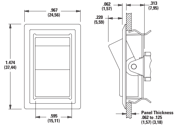
J37 Rocker with Frame
