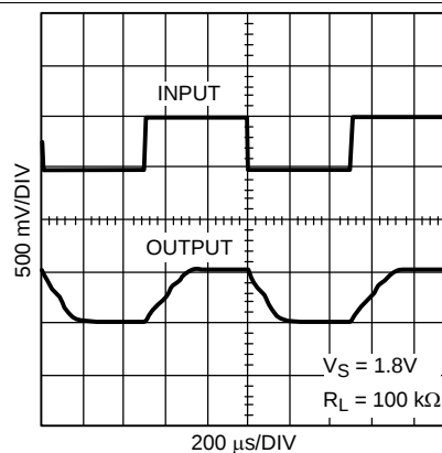
Figure 58. Large Signal Pulse Response
