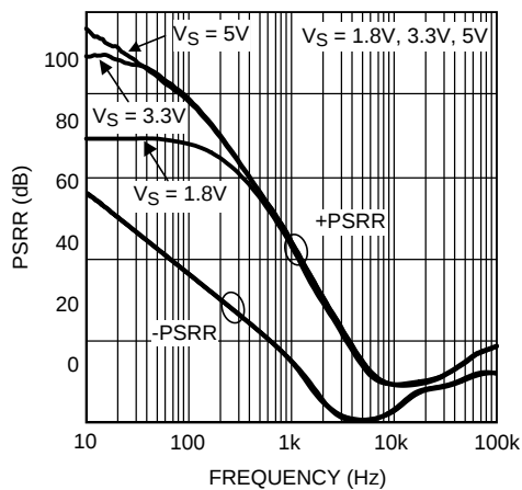
Figure 39. PSRR vs. Frequency
