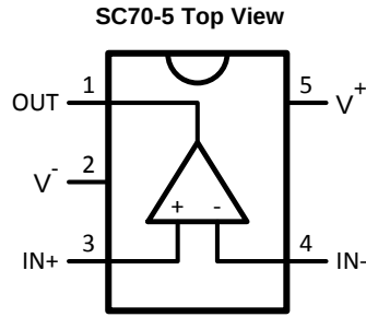
Pin Functions
