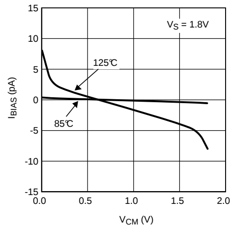
Figure 34. Input Bias Current vs. Common Mode Voltage
