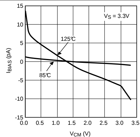
Figure 36. Input Bias Current vs. Common Mode Voltage
