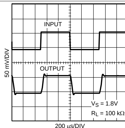
Figure 56. Small Signal Pulse Response
