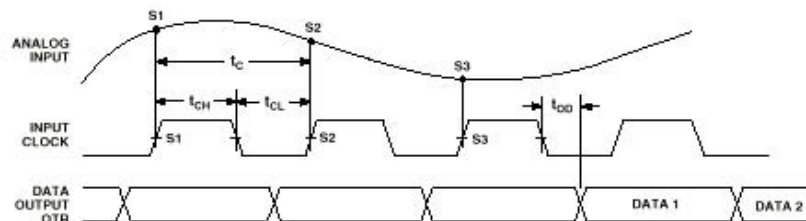
Figure 1. Timing Diagram
