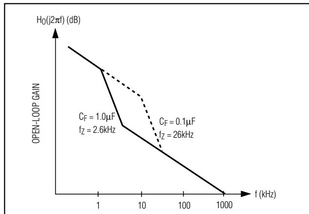
Figure 4. Open-Loop Transfer Function
