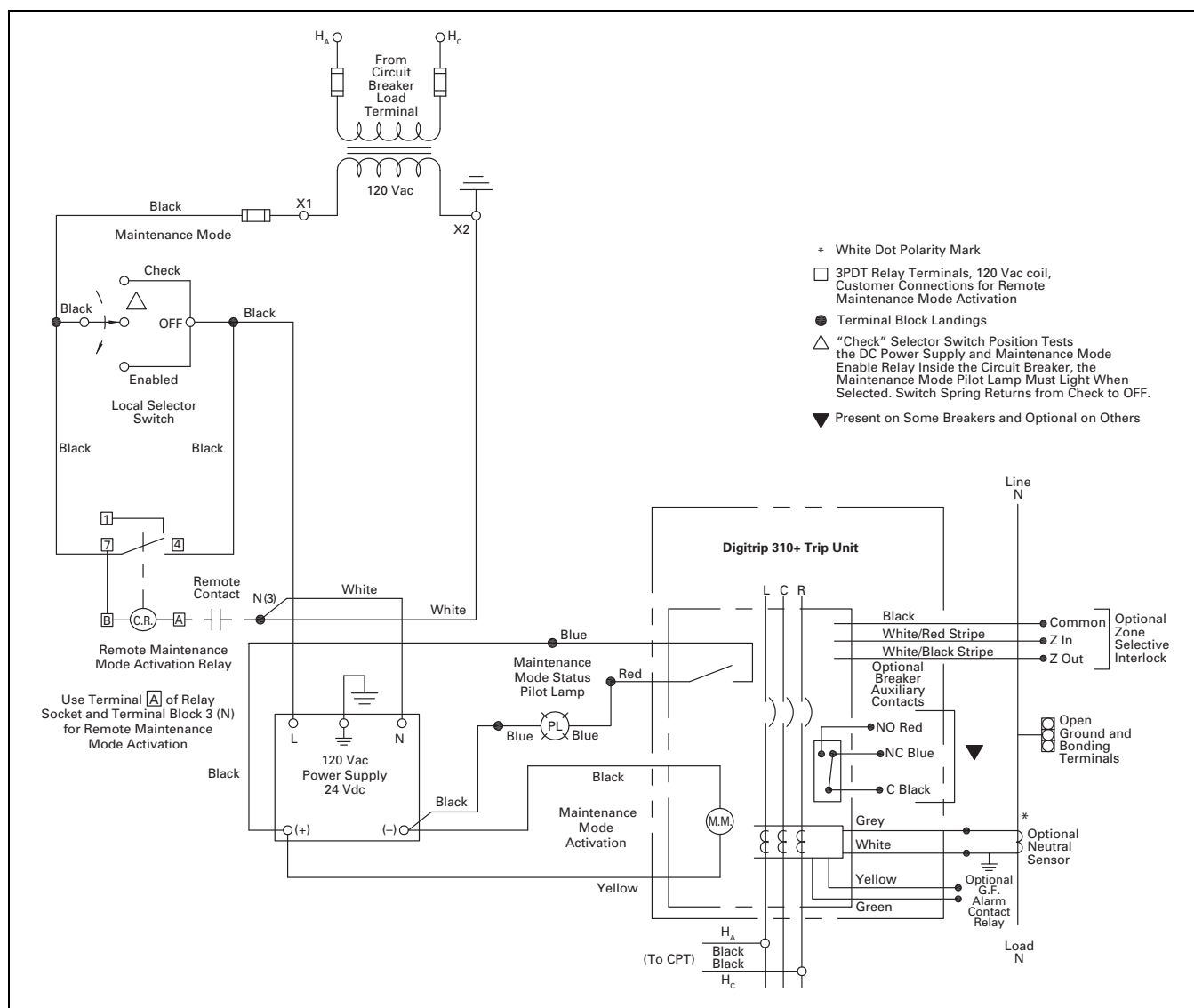
Figure 27.5-1. ECB with Arcflash Reduction Maintenance System Wiring
