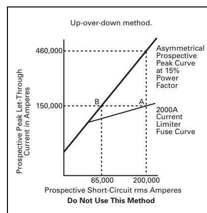
Figure 27.2-4. Up-Over-Down Misapplication
