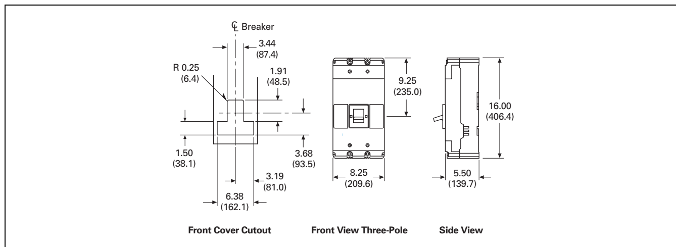
Figure 27.4-8. N-Frame
