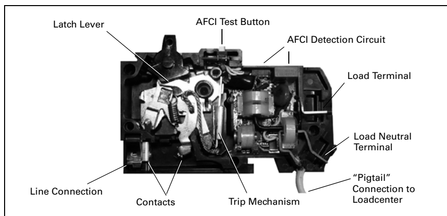
Figure 27.2-5. AFCI Circuit Breaker
