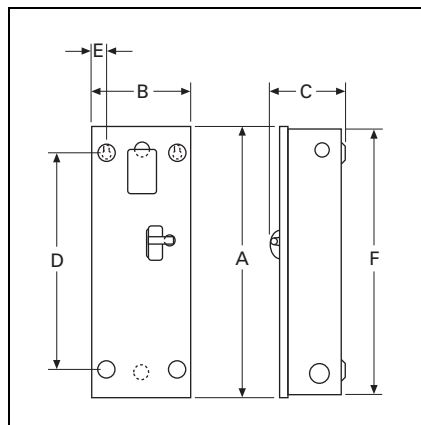
Figure 27.4-16. NEMA 1 Surface Mounted
