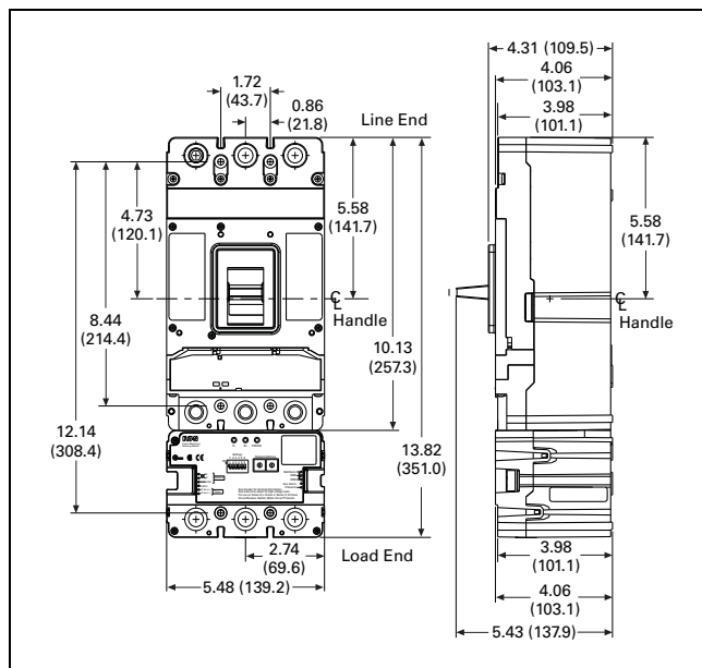
Figure 27.4-12. LG Three-Pole with PM3 Modbus
