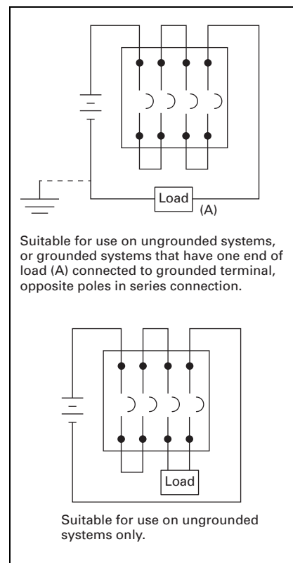
Figure 27.2-8. 750 Vdc Maximum— Four Poles in Series
