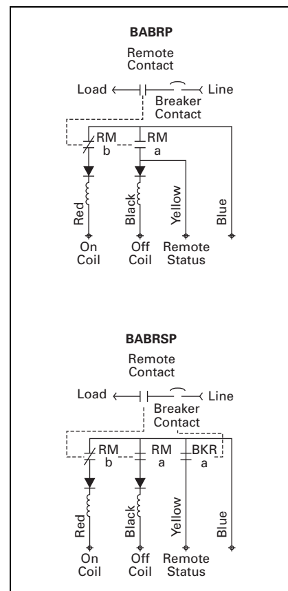
Figure 27.4-1. Control Circuit for the BABRP and BABBSP
