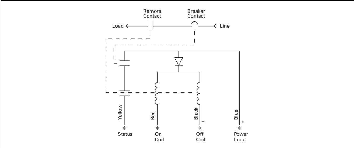
Figure 27.4-5. Typical Circuit Breaker Schematic for GHQRSPEL
