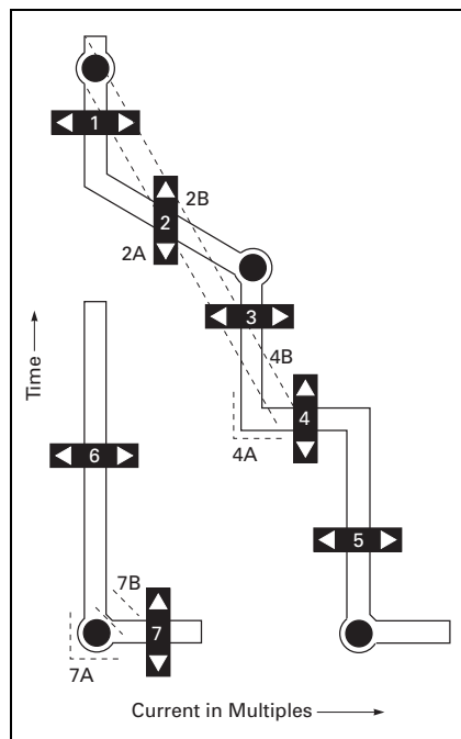
Figure 27.1-1. Time-Current Curve Shaping
