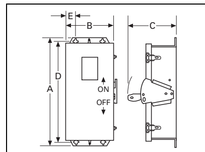
Figure 27.4-21. NEMA 4/4X, 5 Stainless Steel
