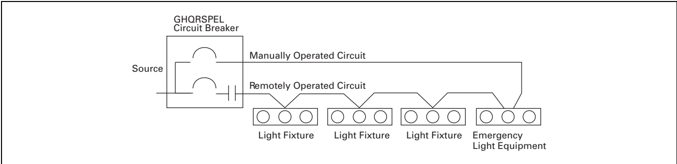
Figure 27.4-4. The Need for Relay is Eliminated with Extra Box, Wiring and Selecting a Properly Rated Component Note: Circuit breaker mounts into panelboard. Switched and unswitched conductors are connected directly to the breaker load side lug.
