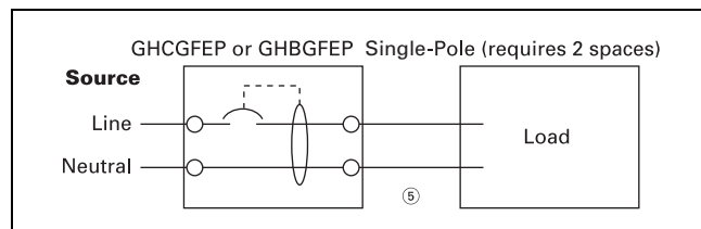
Figure 27.4-6. Electrical Schematic
