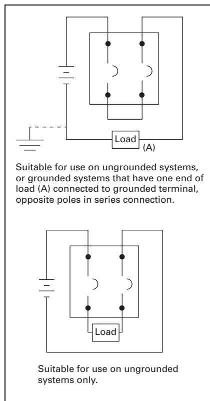
Figure 27.2-6. 250 Vdc Maximum— Two Poles in Series
