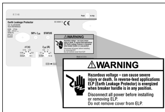
Figure 27.3-12. Earth Leakage Module Suitable for Reverse-Feed Applications
