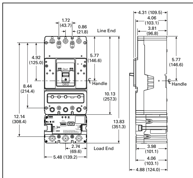
Figure 27.4-11. KD Three-Pole with PM3 Modbus
