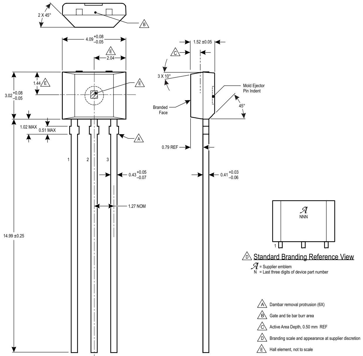
Figure 6: Package UA, 3-Pin SIP, Matrix Style
