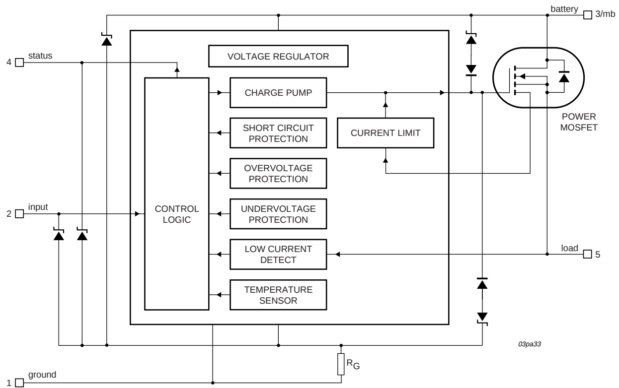
Fig 4. Elements of the high-side TOPFET switch.
