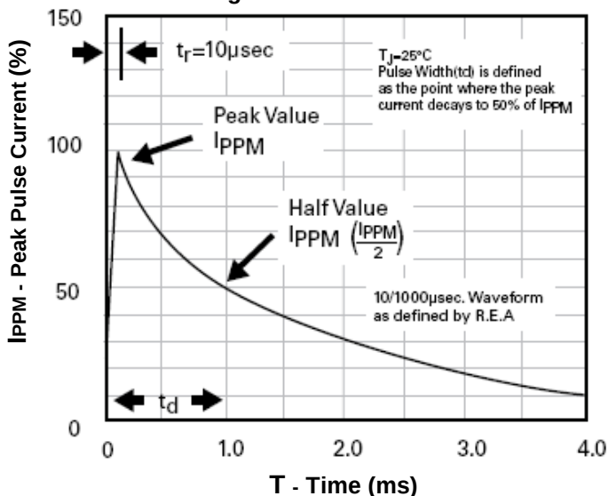
Fig.3- Pulse Waveform
