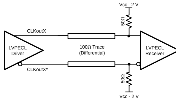
Figure 12. Differential LVPECL Operation, DC Coupling
