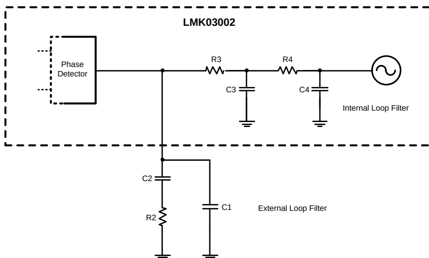
Figure 10. Loop Filter
