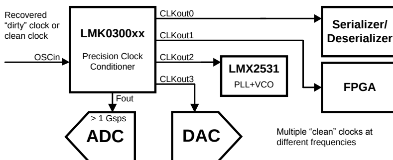
Figure 1. System Diagram
