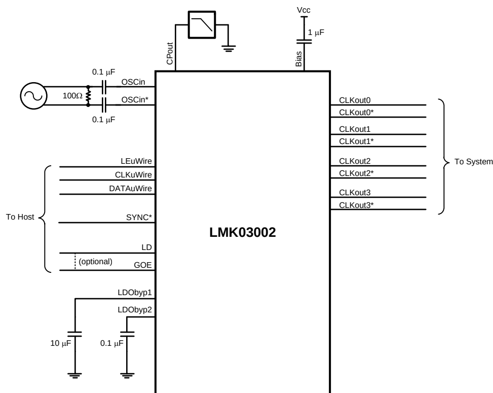
Figure 9. Typical Application
