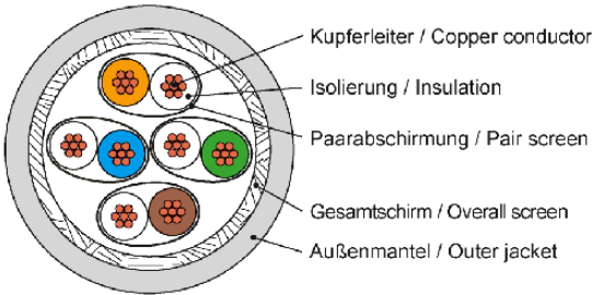
Kabelaufbau / cable design Li-02YSCH 4x2xAWG27/7
