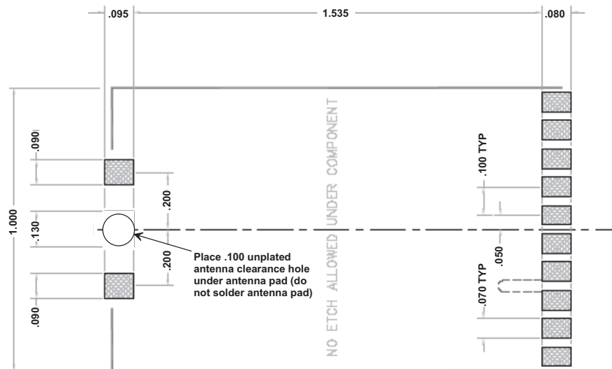
DM1800-916MR-V SMT Mounting Pattern
