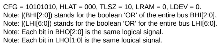
Figure 10-63. Timing Diagram for Devices Above the Winning Device in Block Number 2
