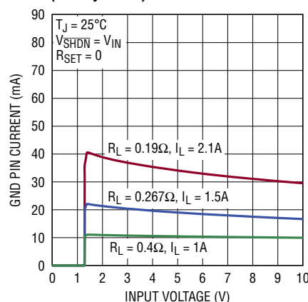
GND Pin Current, V_{OUT} = 0.4\text{V} (Heavy Load)
