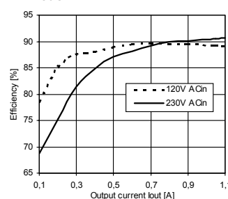
Efficiency (@ V_{out} = 48\text{V} , typ.)
