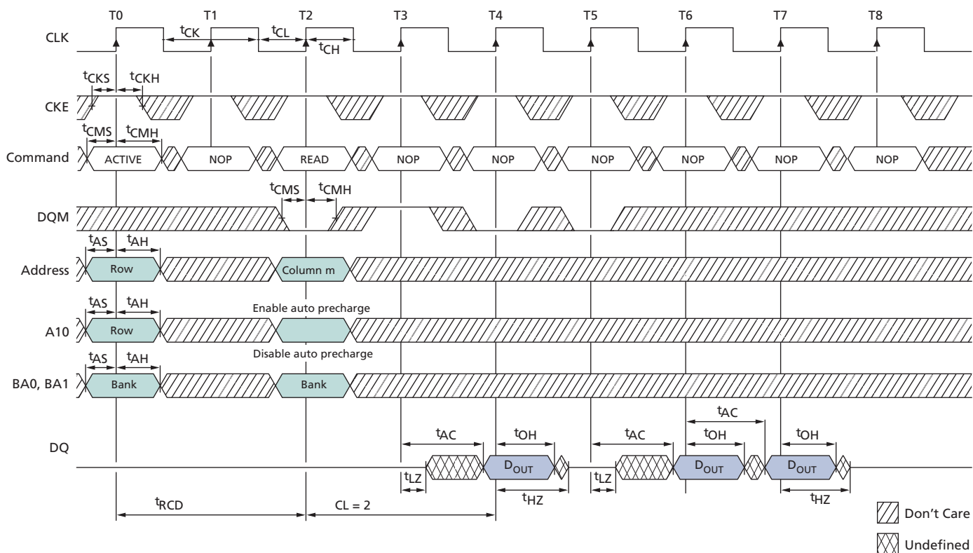
Figure 23: READ – DQM Operation
