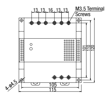
PS5R-F (120W)
