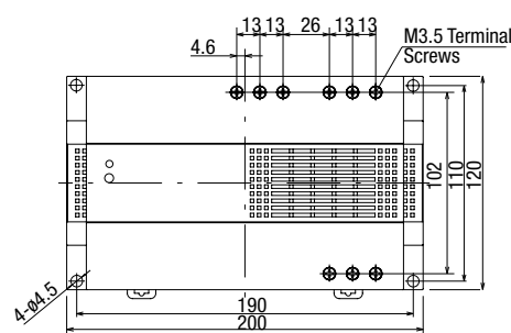
PS5R-G (240W)
