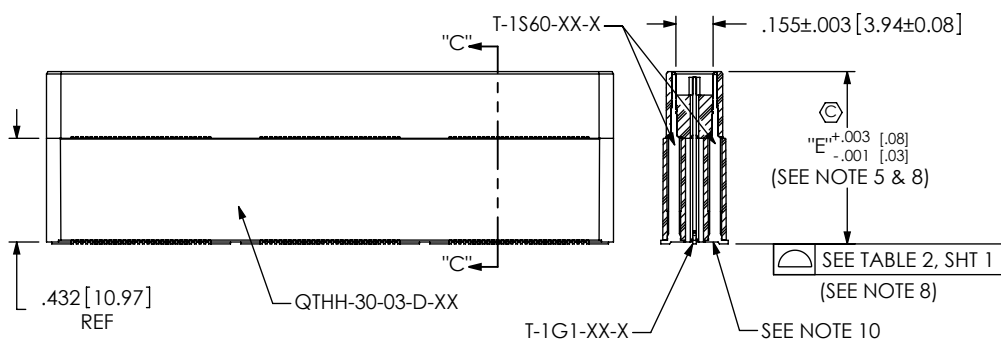
FIG 6 (QTH-090-05-X-D SHOWN) (SAME AS FIG 5, EXCEPT AS SHOWN)
