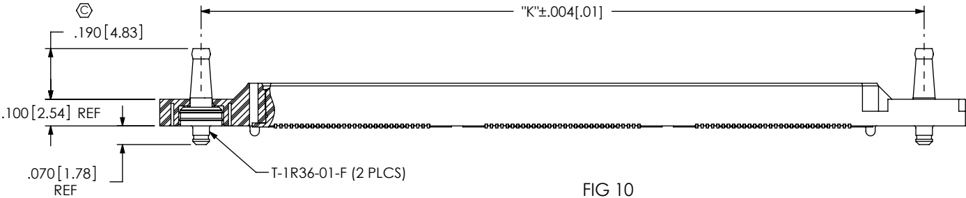
FIG 10 (QTH-090-01-X-D-A-RT1 SHOWN) (NOT AVAILABLE WITH -LC, -GP, OR -FL OPTIONS) (AVAILABLE ON -01 ONLY) (SAME AS FIG 1, EXCEPT AS SHOWN)
