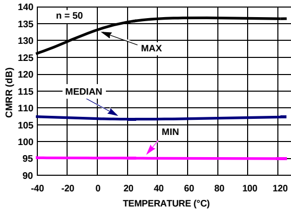
FIGURE 27. CMRR vs TEMPERATURE V_+ = \pm 2.5V, \pm 1.5V
