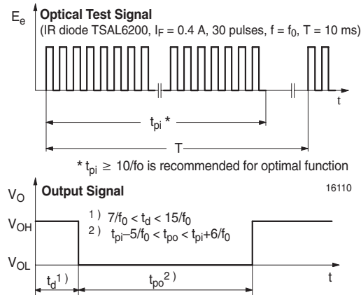
Figure 1. Output Function
