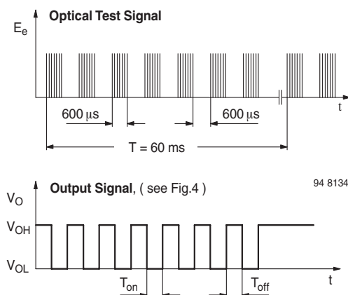
Figure 3. Output Function
