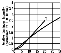
Fig6. RELATIVE LUMINOUS INTENSITY VS. FORWARD CURRENT
