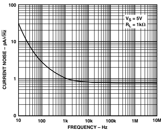
TPC 21. Current Noise vs. Frequency
