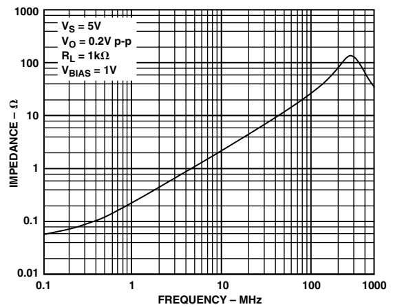
TPC 30. Output Impedance vs. Frequency, V_{OUT} = 0.2 V p-p, R_L = 1 k \Omega , V_S = 5 V
