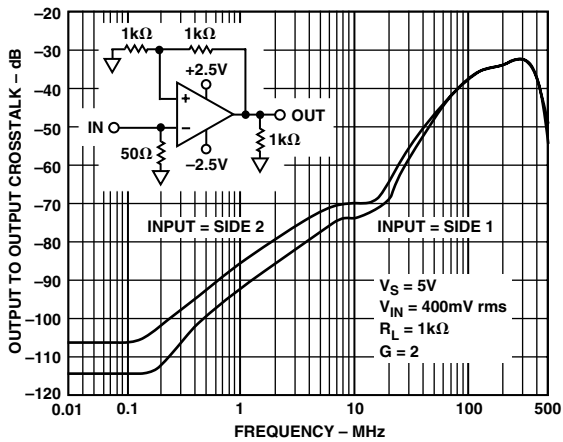
TPC 26. AD8062 Crosstalk, V_{OUT} = 2.0 V p-p, R_L = 1 k \Omega , G = 2 , V_S = 5 V
