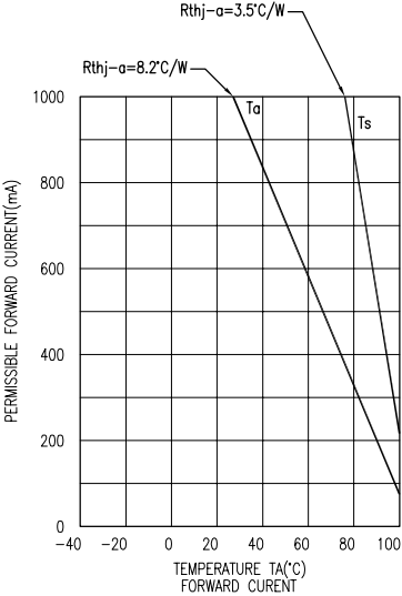
DERATING CURVE
