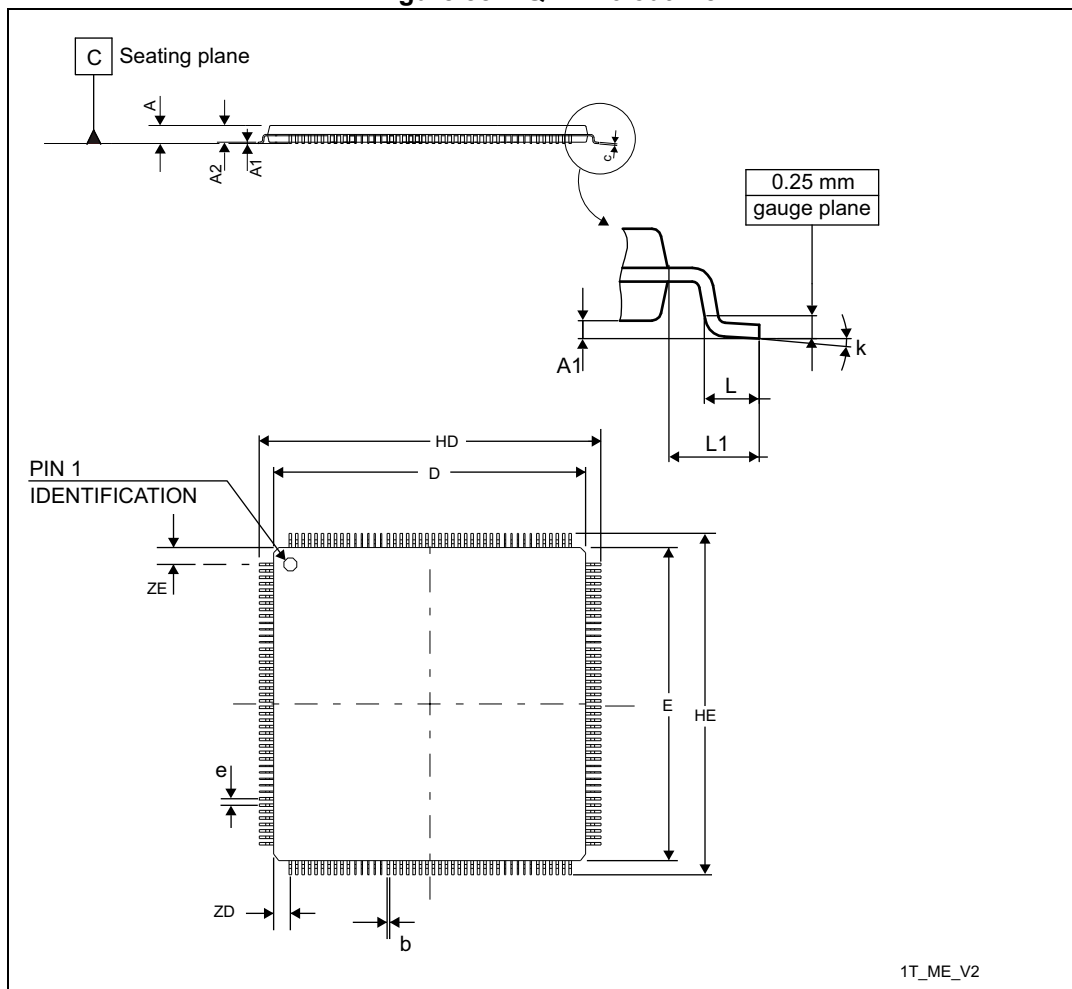
Figure 88. LQFP176 outline
