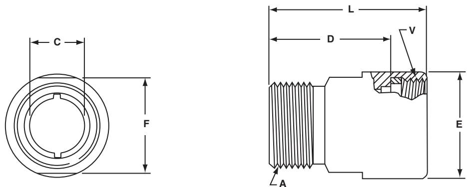
10-113196-XX adapter
