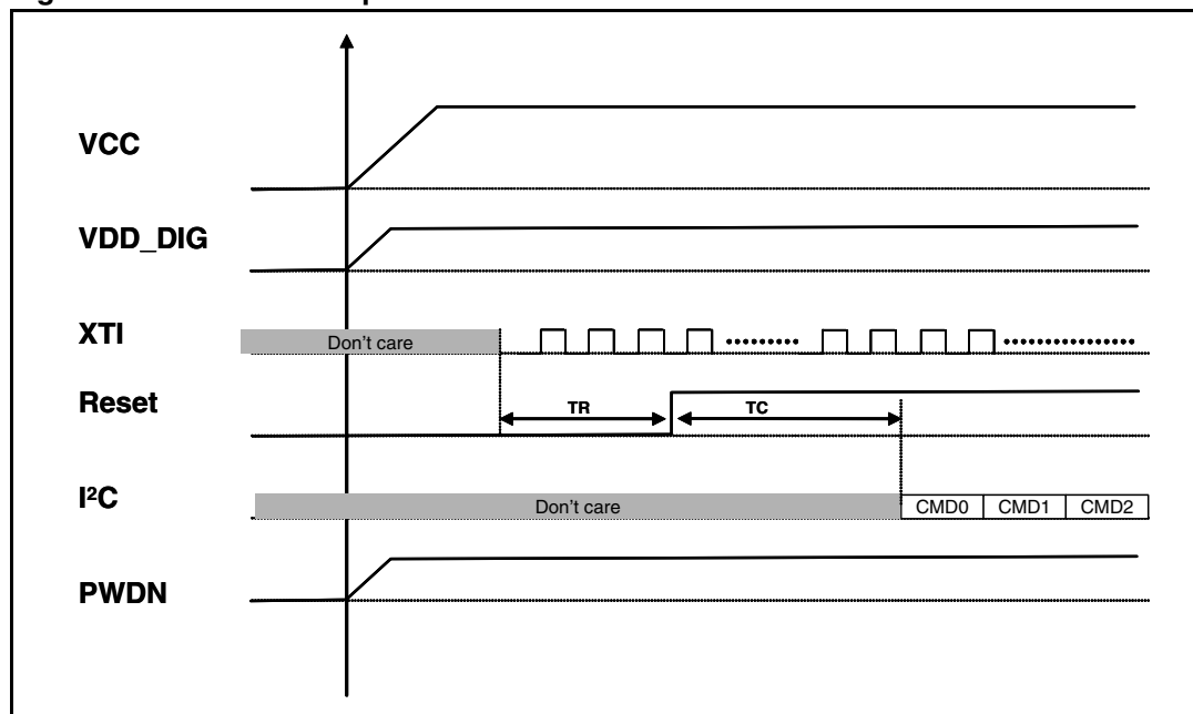
Figure 3. Power-on sequence
