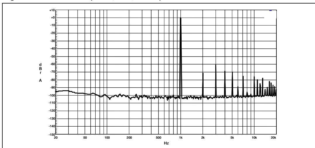
Figure 25. FFT 0 dBfs (1 kHz, 18 V, 8 ohm)
