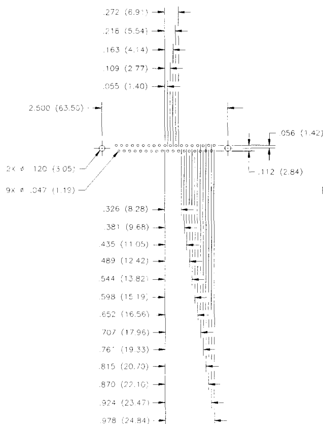
37 Position Shell Size C
