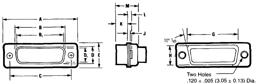
Mating Side
