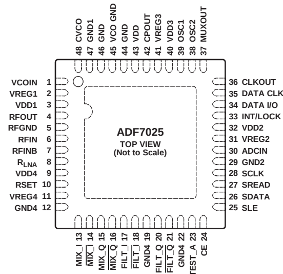
Figure 5. Pin Configuration
