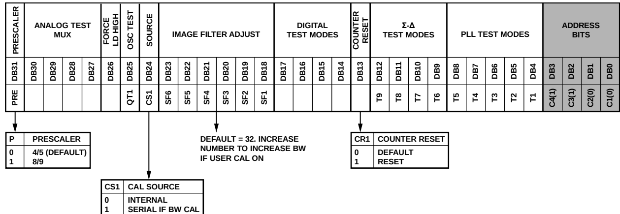
Figure 50. Register 12—Test Register
