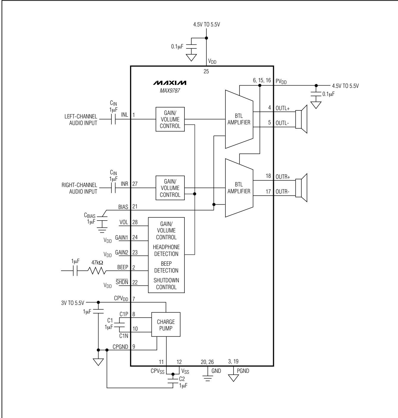
Block Diagram
