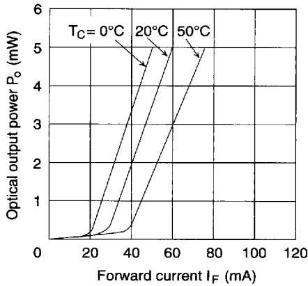
Optical Output Power vs. Forward Current (HL1321AC, HLP5400)
