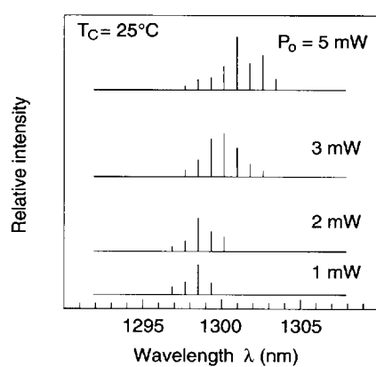
Lasing Wavelength (HL1321AC, HLP5400)
