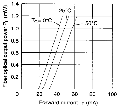
Optical Output Power vs. Forward Current (HL1321BF, DL, DM)
