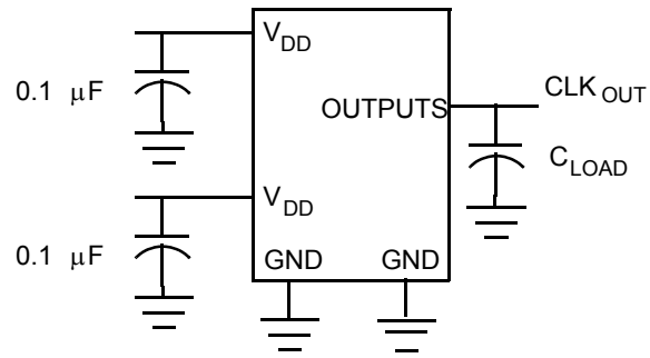
Figure 8. Test Circuit # 1
