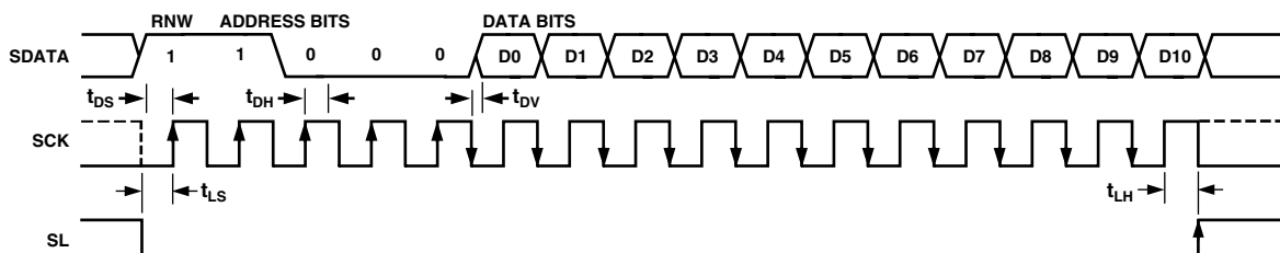
Figure 3. Serial Write Operation
