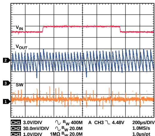
Figure 42. Buck Response to Line Transient, Input Voltage from 4.5 V to 5.0 V, V_{OUT1} = 1.8\text{ V} , I_{OUT1} = 5\text{ mA} , Auto Mode
