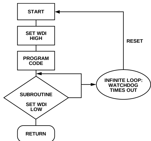
Figure 112. Watchdog Flow Diagram
