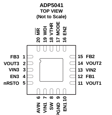
Figure 2. Pin Configuration—View from Top of the Die
