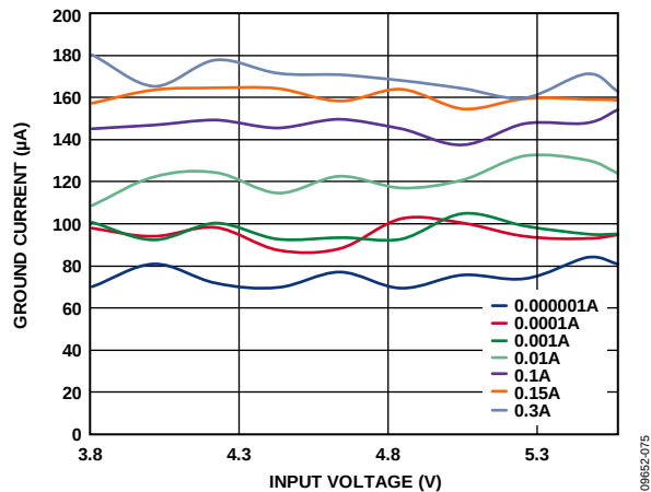
Figure 75. LDO1, LDO2 Ground Current vs. Input Voltage, Across Output Load (A), V_{OUT} = 3.3\text{ V}
