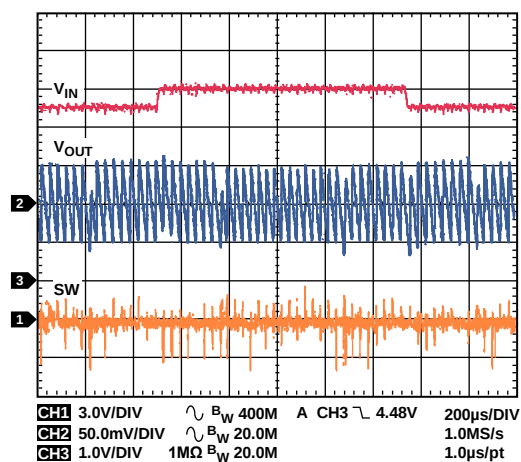
Figure 41. Buck Response to Line Transient, Input Voltage from 4.5 V to 5.0 V, V_{OUT1} = 3.3\text{ V} , I_{OUT1} = 5\text{ mA} , Auto Mode
